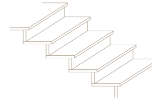
B Classic step construction with riser
